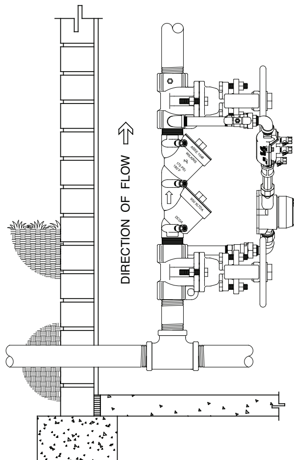
VERTICAL INSTALLATION
