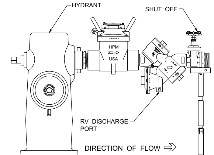
TYPICAL INSTALLATION ZURN WILKINS 975XLHBM Hydrant Backflow Meter
